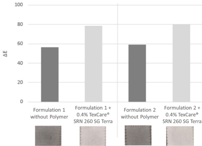
Fig. 3: Improvement of anti-redeposition of a liquid detergent through inclusion of 0.4% a.m. TexCare SRN 260 Terra on polycotton. Tergotometer, 25°C for 30 min, 2 g/L liquid detergent, 0.08 g/L olive oil-carbon black soil.
